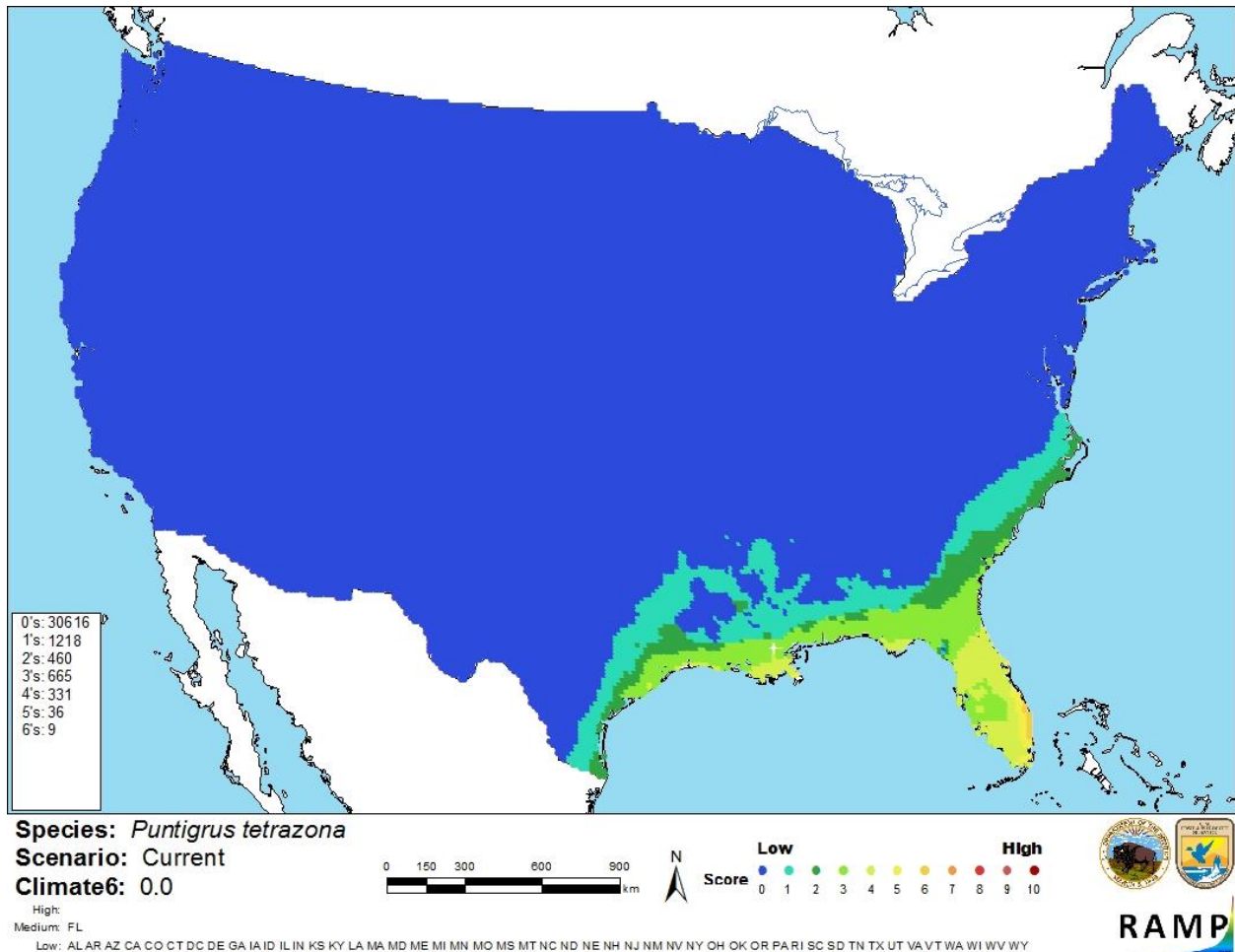
Figure 4. Map of RAMP (Sanders et al. 2014) climate matches for Puntigrus tetrazona in the contiguous United States based on source locations reported by GBIF Secretariat (2018) and Nico et al. (2018). 0= Lowest match, 10=Highest match.
